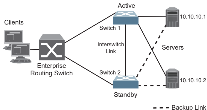
Figure 56. Hot-Standby Redundancy
