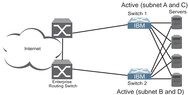
Figure 61. Active-Active Redundancy
