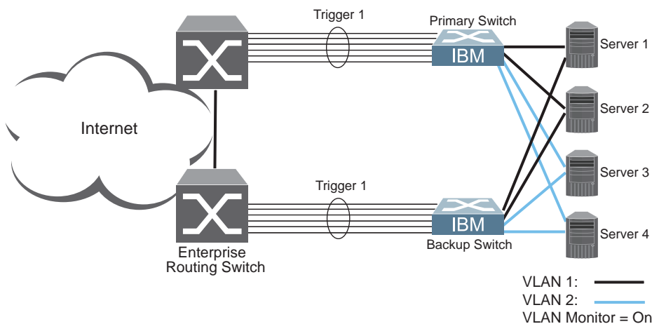
Figure 57. Basic Layer 2 Failover
