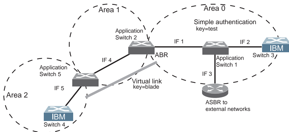
Figure 50. OSPF Authentication
