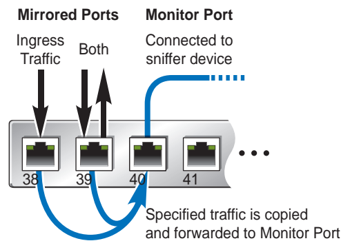
Figure 65. Mirroring Ports
