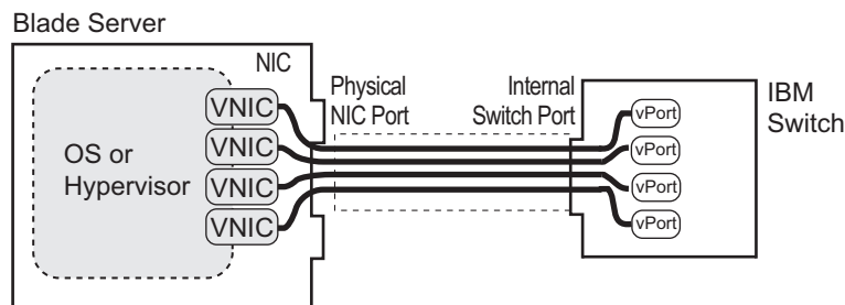
Figure 37. UFP vPorts
