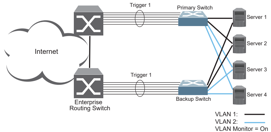
Figure 55. Basic Layer 2 Failover
