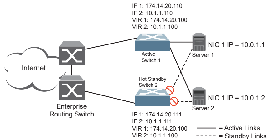
Figure 62. Hot-Standby Configuration
