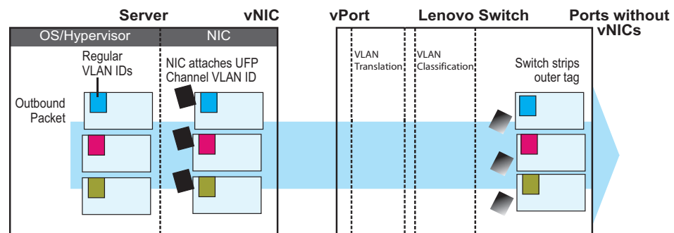
Figure 37. Packet passing through in Trunk Mode
