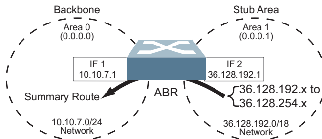
Figure 51. Summarizing Routes
