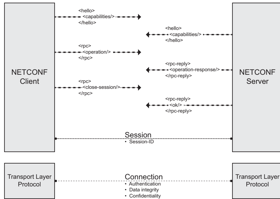
Figure 63. NETCONF Operations Procedure
