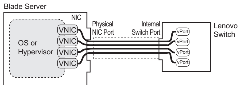
Figure 35. UFP vPorts
