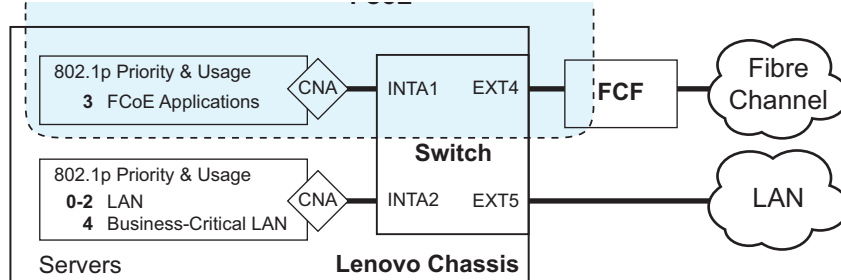
Figure 32. A Mixed Fibre Channel and FCoE Network
