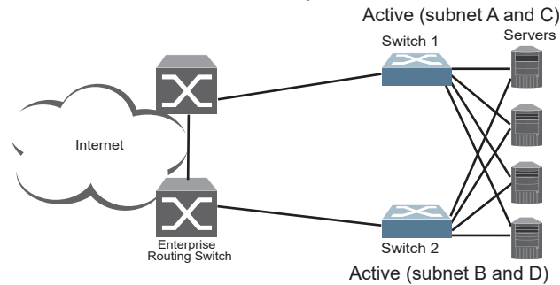
Figure 59. Active-Active Redundancy
