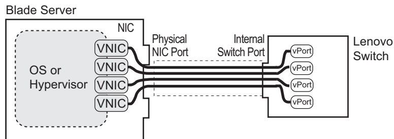
Figure 34. UFP vPorts
