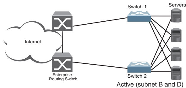
Figure 58. Active-Active Redundancy
