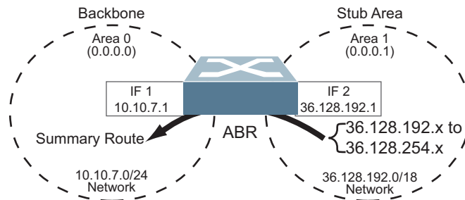
Figure 50. Summarizing Routes
