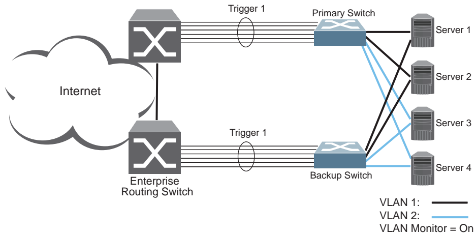
Figure 54. Basic Layer 2 Failover
