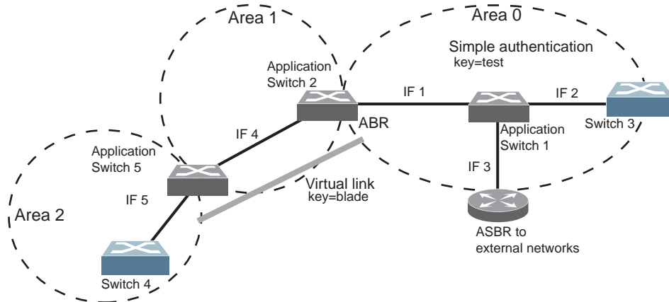
Figure 47. OSPF Authentication
