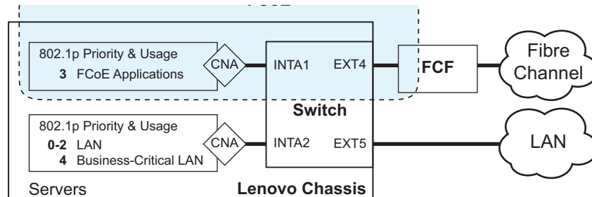
Figure 31. A Mixed Fibre Channel and FCoE Network
