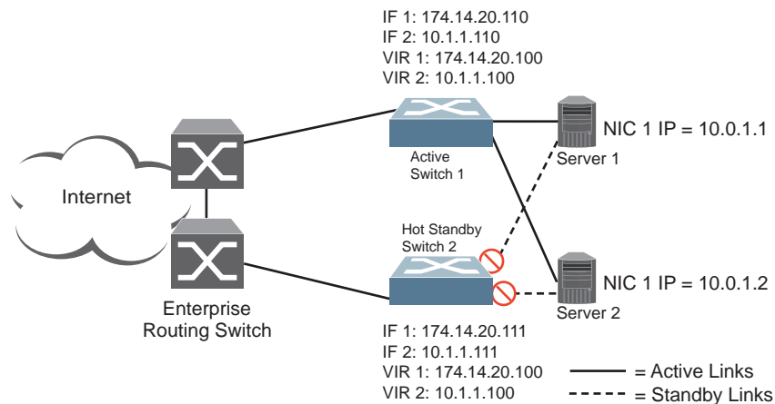
Figure 61. Hot-Standby Configuration
