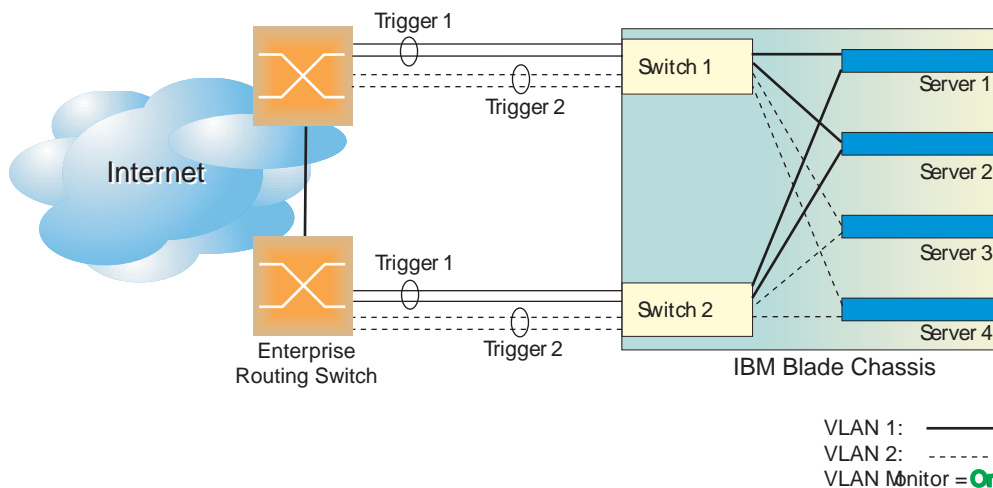
Figure 48. Two trunks, each in a different Failover Trigger
