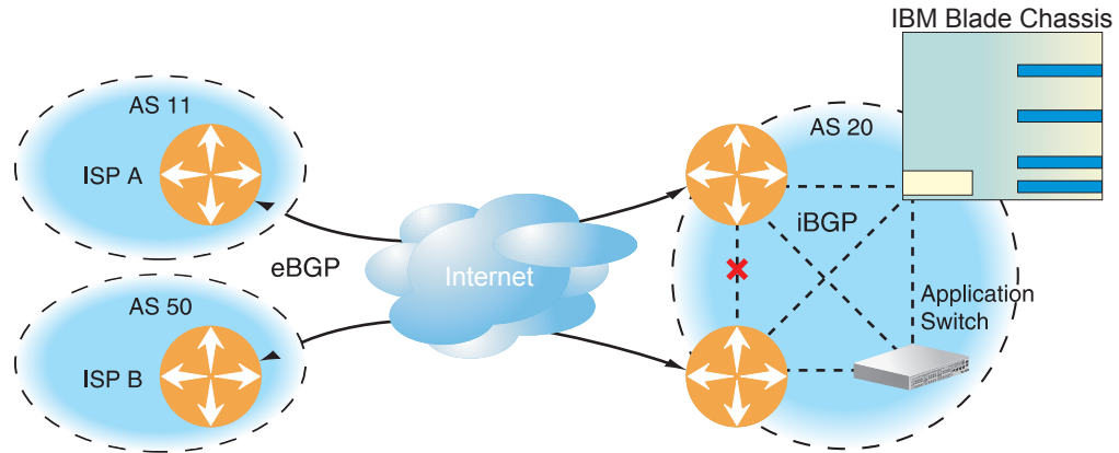
Figure 33. iBGP and eBGP
