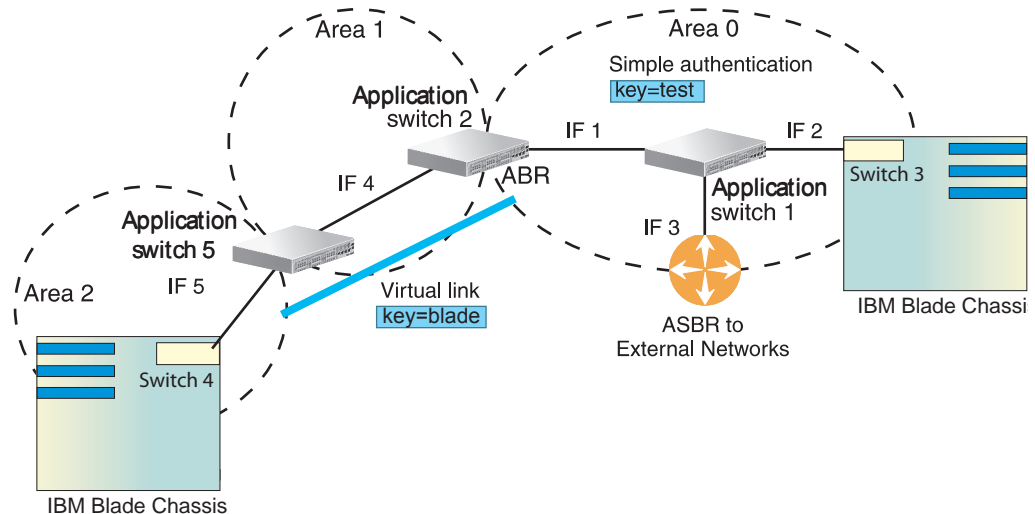
Figure 40. OSPF Authentication
