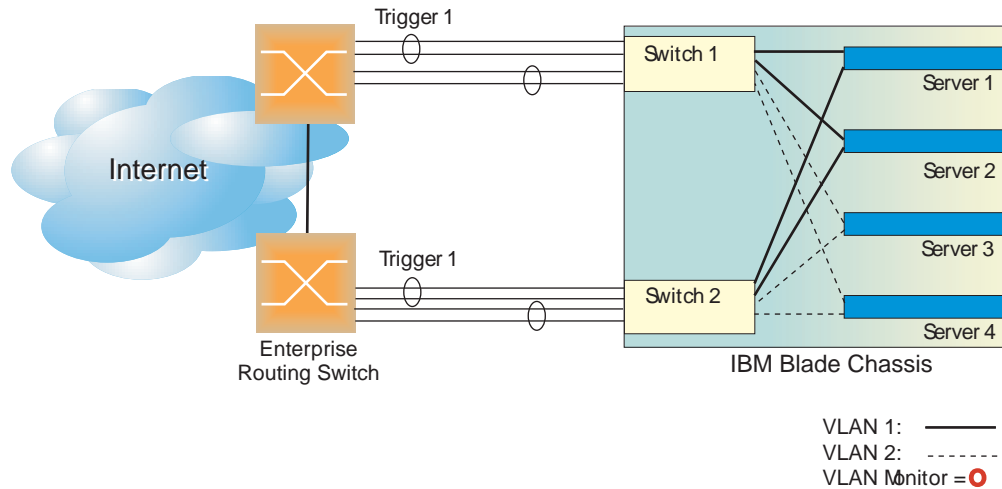
Figure 49. Two trunks, one Failover Trigger
