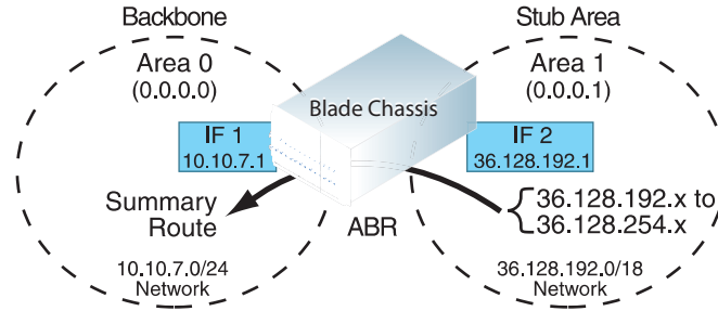
Figure 43. Summarizing Routes
