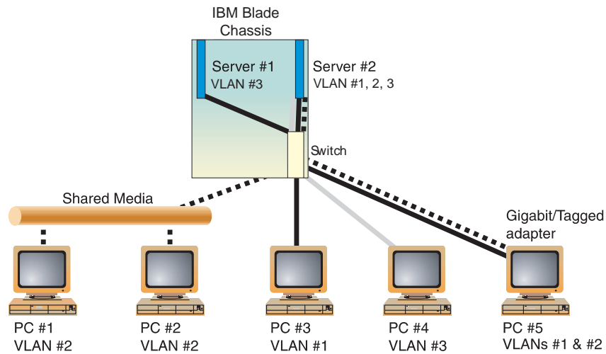
Figure 7. Multiple VLANs with VLAN-Tagged Gigabit Adapters
