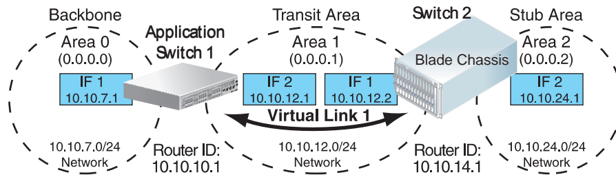
Figure 42. Configuring a Virtual Link
