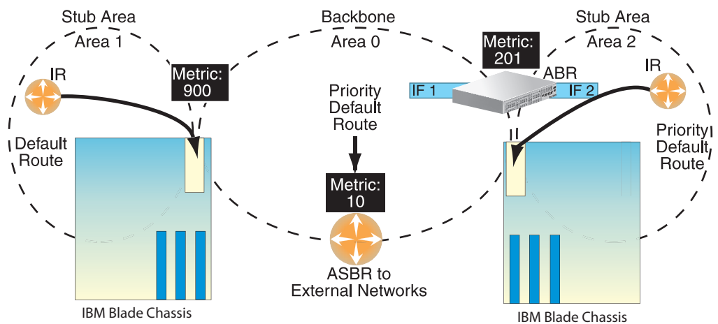
Figure 39. Injecting Default Routes
