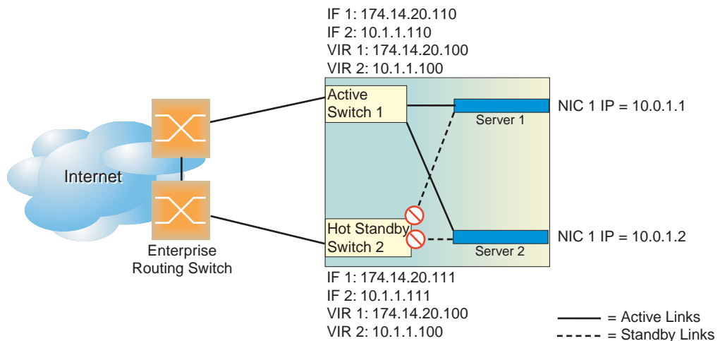
Figure 54. Hot-Standby Configuration
