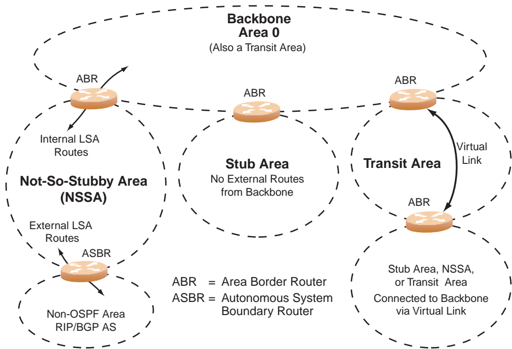
Figure 37. OSPF Area Types
