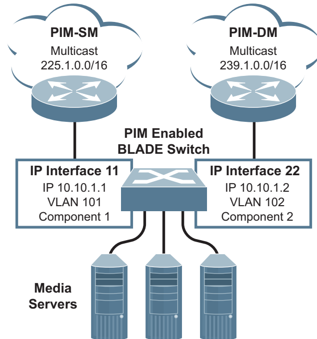
Figure 45. Network with both PIM-DM and PIM-SM Components
