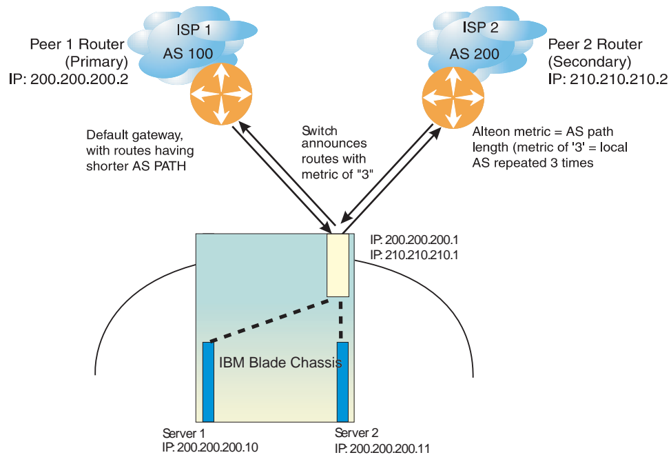
Figure 35. BGP Failover Configuration Example
