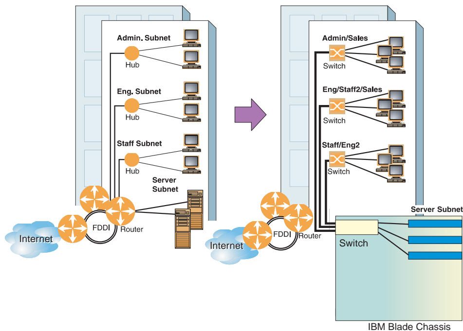
Figure 29. The Router Legacy Network
