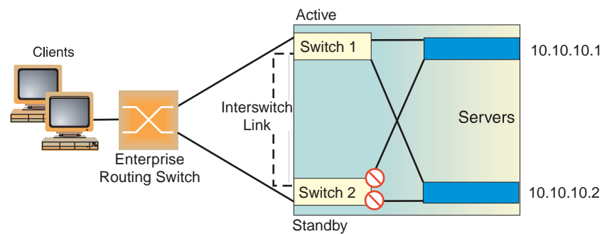
Figure 52. Hot-Standby Redundancy
