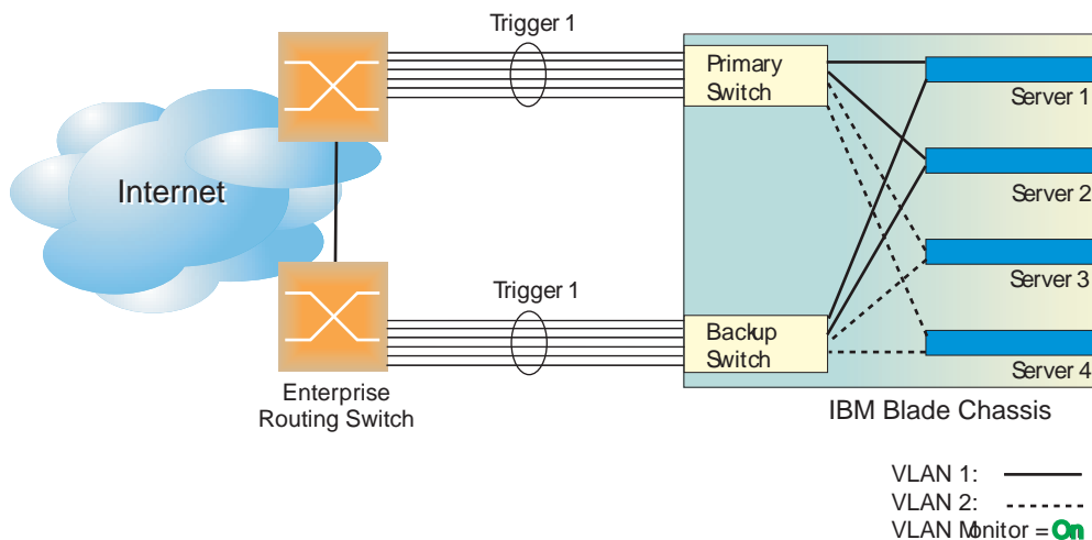
Figure 47. Basic Layer 2 Failover
