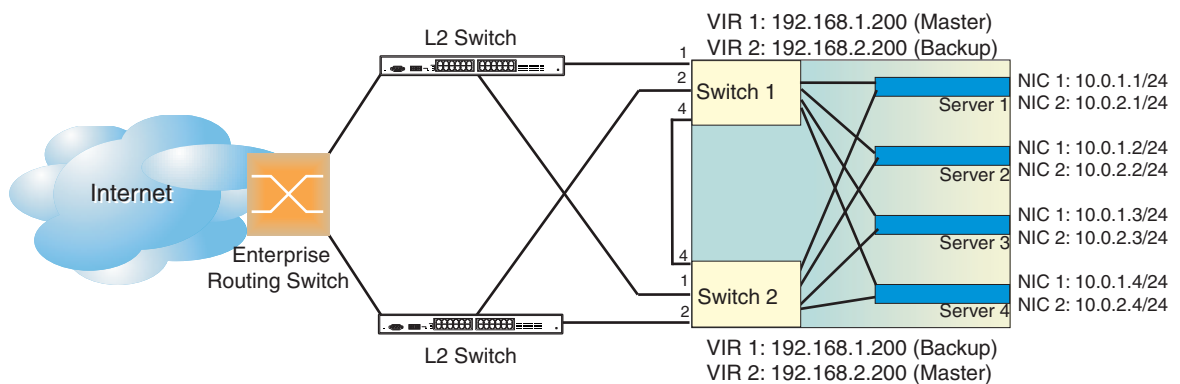
Figure 53. Active-Active High-Availability Configuration
