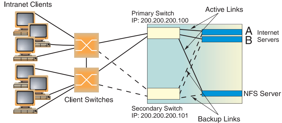
Figure 50. A Non-VRRP, Hot-Standby Configuration
