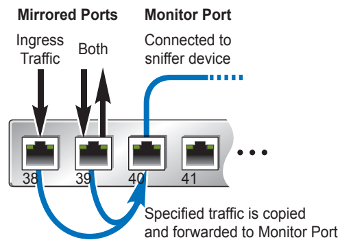
Figure 55. Mirroring Ports
