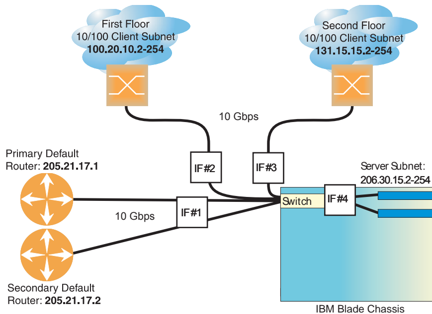
Figure 30. Switch-Based Routing Topology
