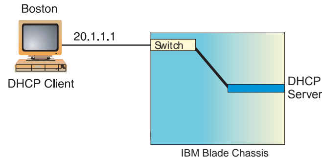
Figure 32. DHCP Relay Agent Configuration
